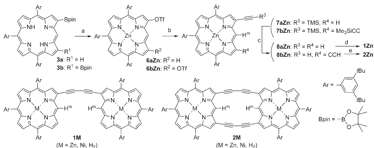
Scheme 1. Synthesis of diporphyrins 1 and 2 . Reaction conditions: a) 1) Oxone, THF/acetone/H 2 O, RT, 1.5 h; 2) PhNTf 2 , Cs 2 CO 3 , DMF, RT, 12 h; 3) Zn(OAc) 2 , CHCl 3 , MeOH, RT, 2 h; b) Me 3 SiCCH, [Pd(PPh 3 ) 4 ], CuI, Et 3 N, DMF, toluene, 70 °C, 3 h; c) K 2 CO 3 , THF, MeOH, RT, 2 h; d) Cu(OAc) 2 , toluene, pyridine, RT, 24 h; e) Cu(OAc) 2 , THF, pyridine, RT, 24 h. Tf: trifluoromethanesulfonyl; DMF: N,N -dimethylformamide; TMS: trimethylsilyl.
